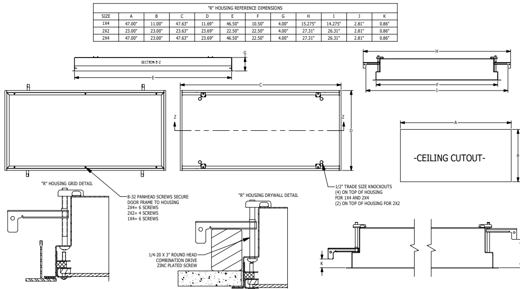
01-AA-L-STD REC CHANNEL DWG. DATE: 12/14/2020
