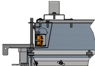
Grid Installation Detail
