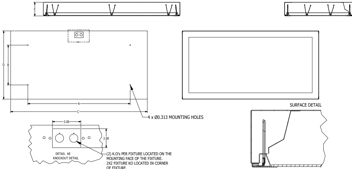
01-CC-L-EZ SURF OVERLAPPING DWG. DATE: 12/22/2020
