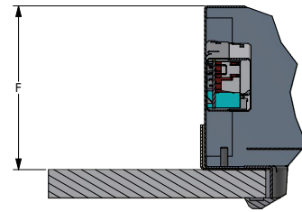
DRYWALL SECTION VIEW
